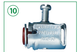
10 Size: 3/8": P/N E00-003-003 1/2": P/N E00-004-003 Type: Speed Lock Style, Snap-in Material: Steel Insulated: Yes
