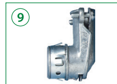
9 Size: 3/8": P/N E00-015-000 1/2": P/N E00-005-001 Type: Snap-in, 90° Material: Die Cast Insulated: No
