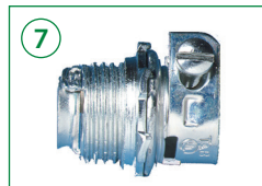
7 Size: 3/8": P/N E00-041-001 Type: Set Screw, Squeeze Material: Steel Insulated: No
