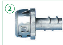
2 Size: 3/8": P/N E00-003-000 1/2": P/N E00-005-000 Type: Screw-in/Snap-in Material: Die Cast Insulated: Yes or No (circle one)
