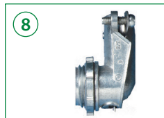
8 Size: 3/8": P/N E00-007-000 1/2": P/N E00-010-000 Type: Set Screw, 90° Material: Die Cast Insulated: Yes or No (circle one)
