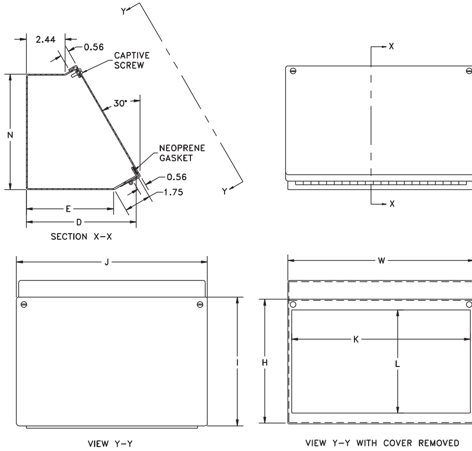
VIEW Y-Y
