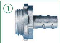
1 Size: 3/8": P/N E00-001-000 1/2": P/N E00-026-000 Type: Screw-in Material: Die Cast Insulated: Yes or No (circle one)
