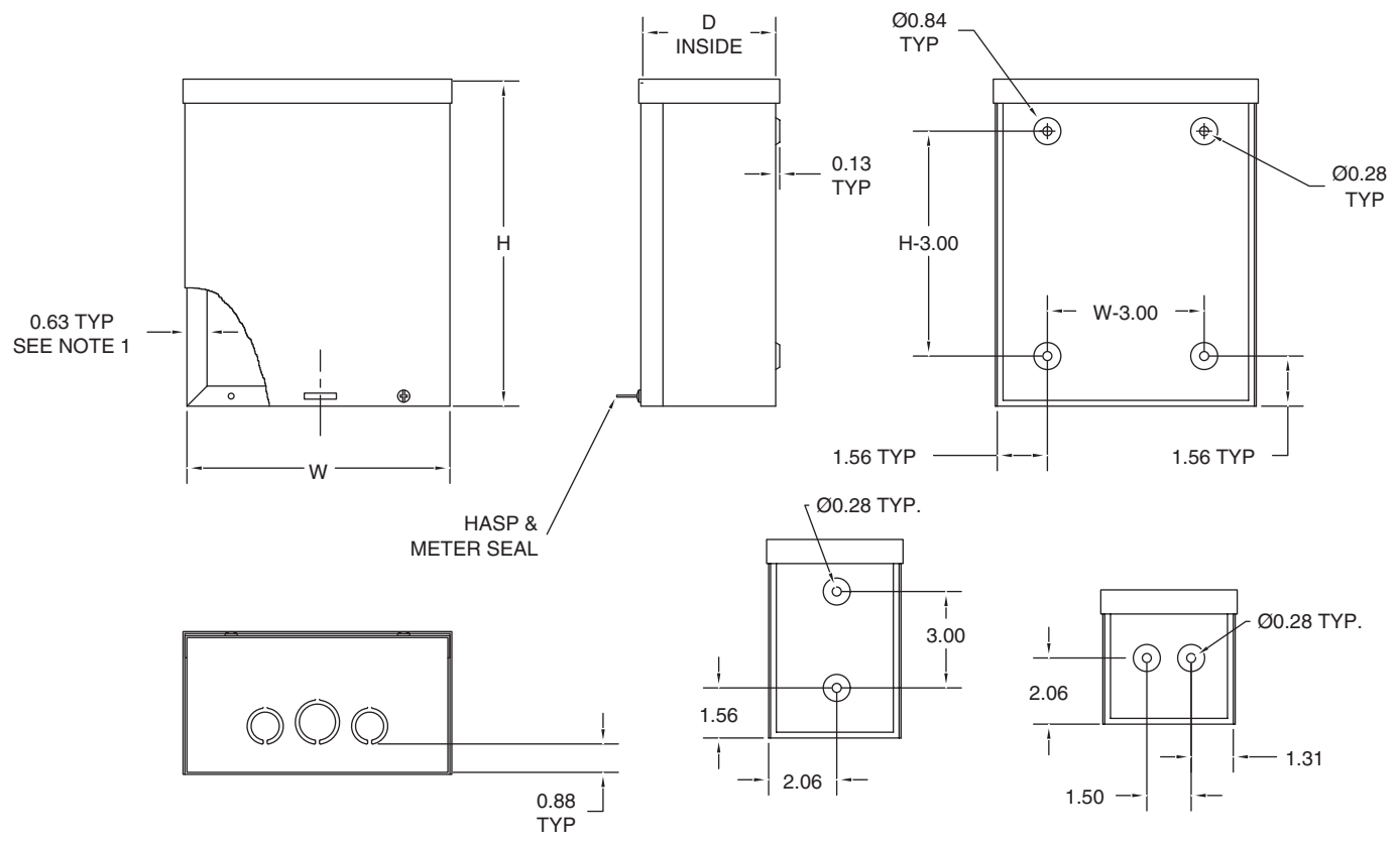
4.00" X 6.00" MOUNTING
