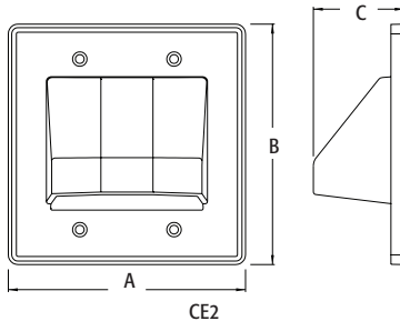
CE2 with SCOOP facing IN CE2 with SCOOP facing OUT
